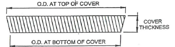
CUT-AWAY VIEW OF EXISTING FRAME & COVER
